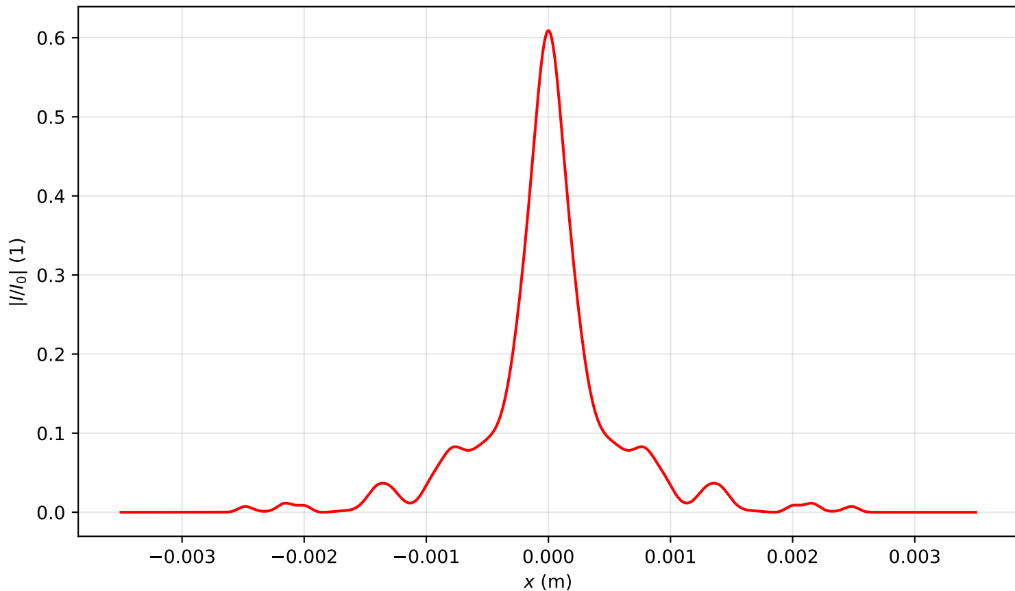
Intensity profile I(x, y = 0, z = 2.388)/I_0 , P_{in}=5.0P_{cr} , artificial time
